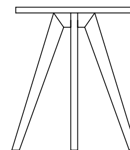
Timber base example
